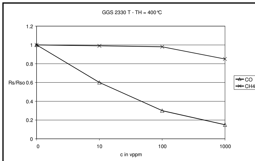
Figure 1: Sensitivity characteristics to impact at CO and CH 4
