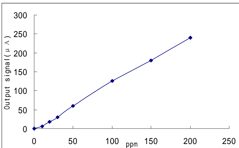
Chart 2 .sensitivity curve
