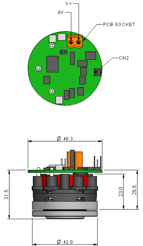
All dimensions in mm All tolerances ±0.15 mm unless otherwise stated
