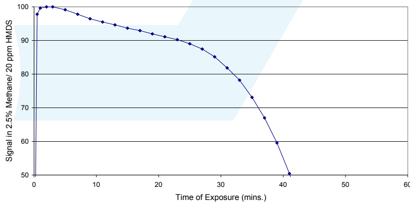
Accelerated Life Tests 4P-75 HMDS Poison Resistance
